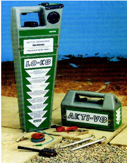
C.A.T & GENERATOR
